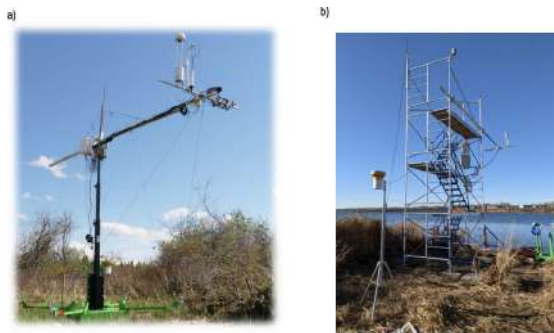
Fig. 1 a) is a photo of the old instrumentation tower installed in April 2020 and b) is a photo of the new instrumentation tower installed in September 2021.
