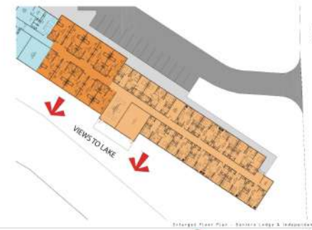
Enlarged Floor Plan - Senior Lodge & Independent Living Wing November 27, 2021 THE WORKLIN GARRICK PARTNERSHIP Alexis Pasa Tibi Care Facility A.26
